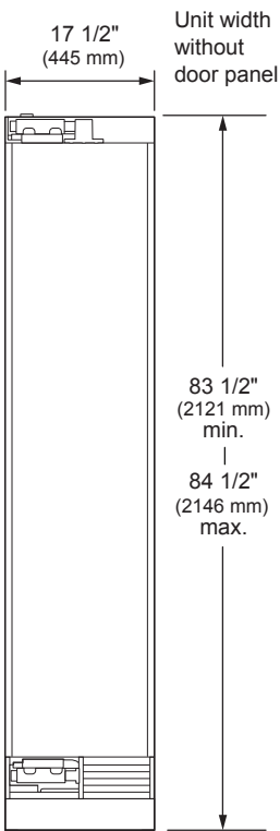
FRONT VIEW
